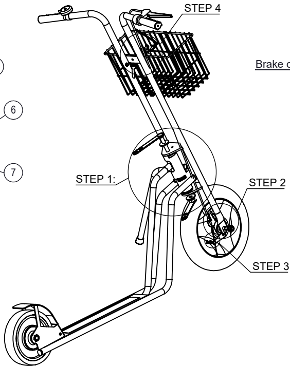
STEP 1: Attach front part to rear part
