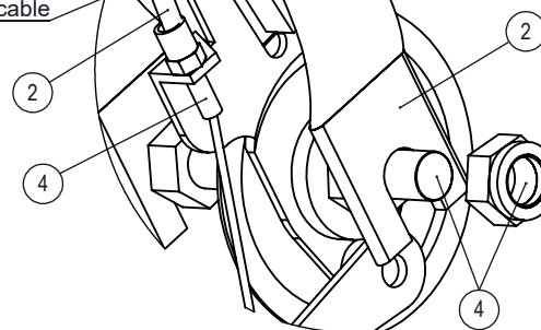
STEP 2: Attach wheel to front part
