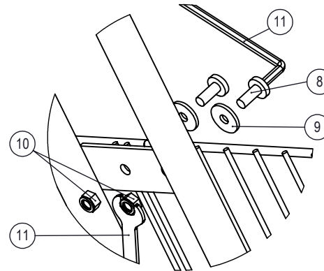
STEP 4: Attach basket to front part
