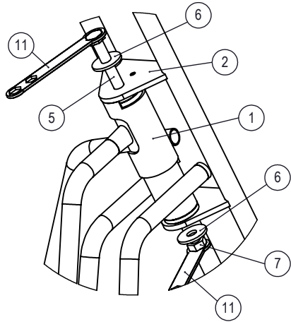
STEP 1: Attach front part to rear part
